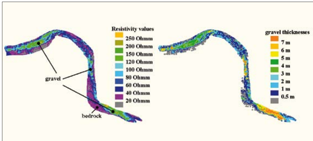
Figure 5: The derived gravel thicknesses.
