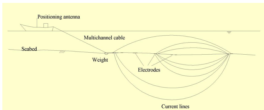
Figure 2 Principles of Vertical Electrical Sounding – On water
