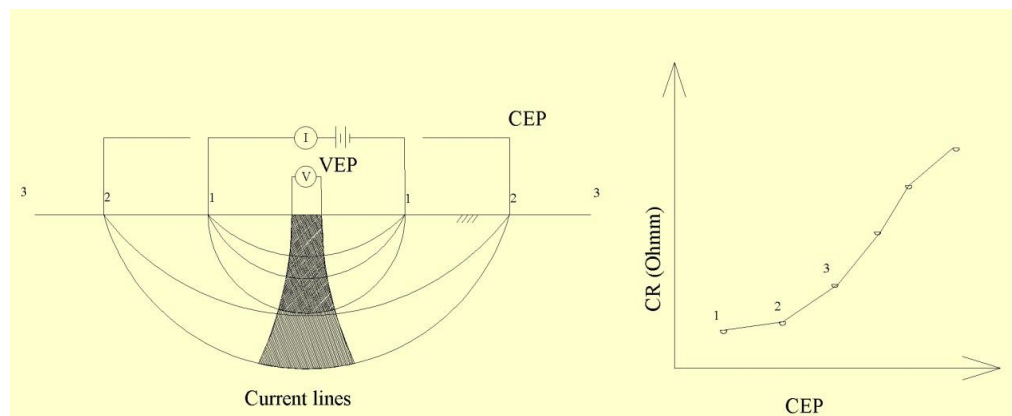
Figure 1 Principles of Vertical Electrical Sounding – On land. Left: a typical land base setup for a resistivity survey. The VEPs are placed between the CEP. Current and voltage measured at the VEP is used to derive the Calculated Resistivity (CR). Right: a typical resistivity curve for a given injection of current as a function of CEP (X axis) and CR (Y axis).
