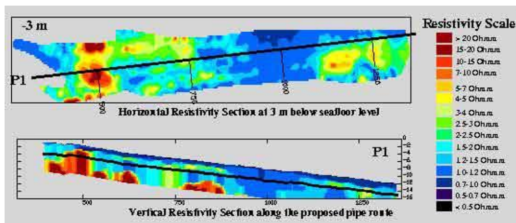
Figure 3 Horizontal and vertical resistivity sections from a pipe route survey in Ireland.
