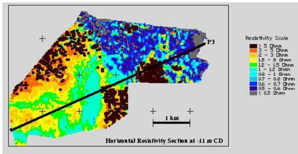
Figure 4 The results of the JNPT port pre-construction survey allowed engineers to visualise the sub-bottom structures and take advantage of the paleo-channel (light blue) and paleo-delta areas (dark blue) to locate channels and vessel turning areas resulting in substantially reduces dredging costs.
