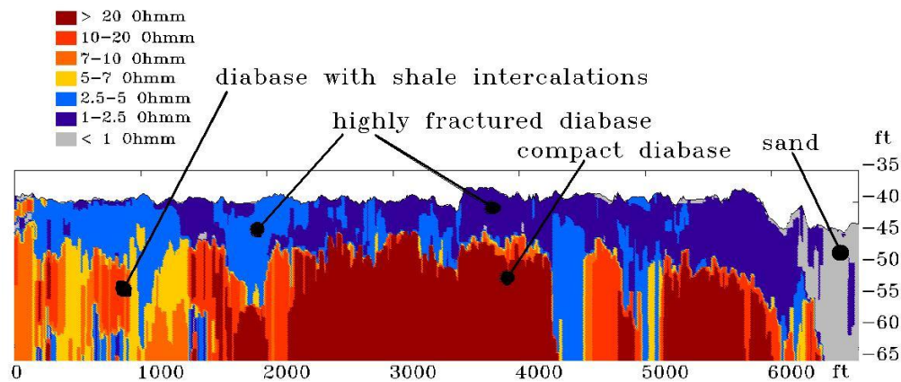
Figure 5: Highly fractured rock overlying less fractured rocks as a result of previous blast dredging.
